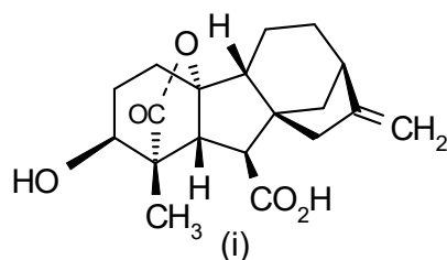
( i ) C 19 H 24 O 5 (분자량: 332.4)
